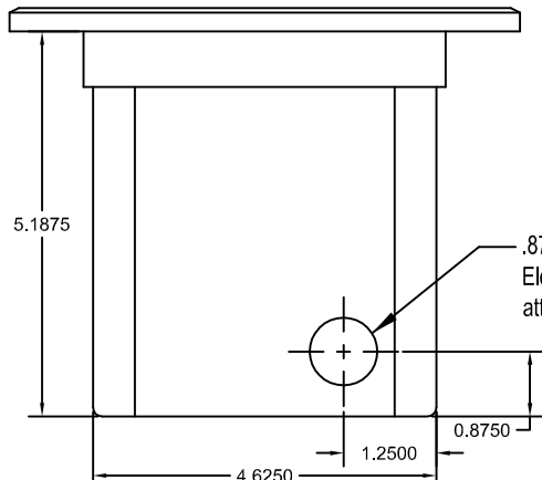
IAF1 Power Box Assembly
